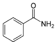
Molecule 1
