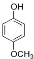
Molecule 7
