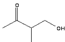
Molecule 9
