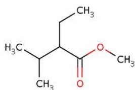
Molecule 3
