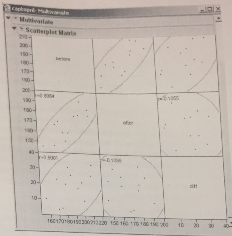
Figure 1: Scatterplot matrix for the variables before , after , and diff .
